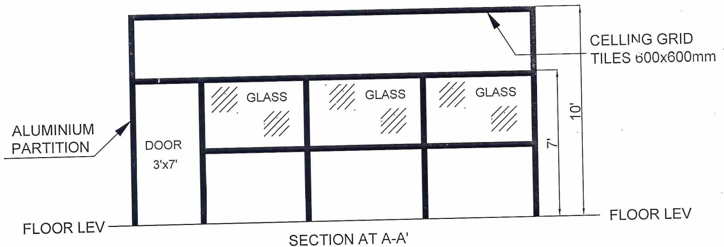
TOOL STORE & STORE OFFICE PROPOSED LAYOUT
